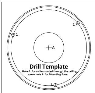
Figure 2-3 Drill Template
