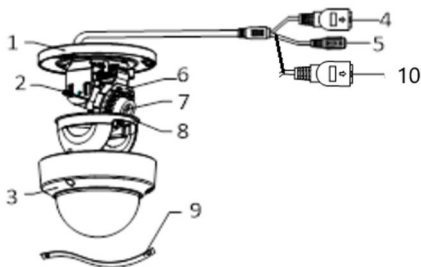
Figure 1-1 Camera Overview
