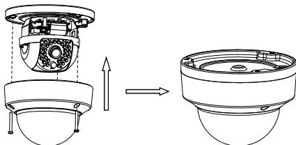
Figure 2-9 Bubble Reinstallation
